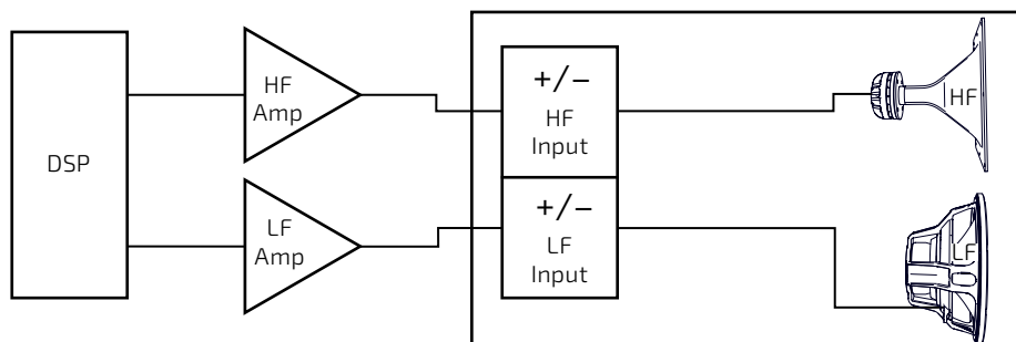
Two-way biamp
